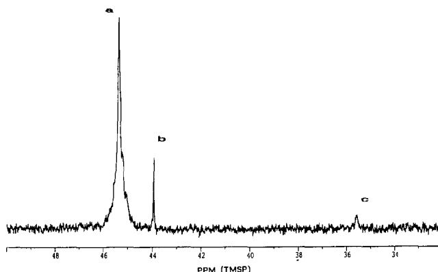
Fig. 1. ^{13}\text{C} NMR spectra at 150 MHz of ^{13}\text{C} dimethylated apo AI at pH 7.7. The upfield region of the proton decoupled ^{13}\text{C} NMR spectra obtained at 4°C for apo AI (2 mg/ml, 24000 acquisitions) are shown.
